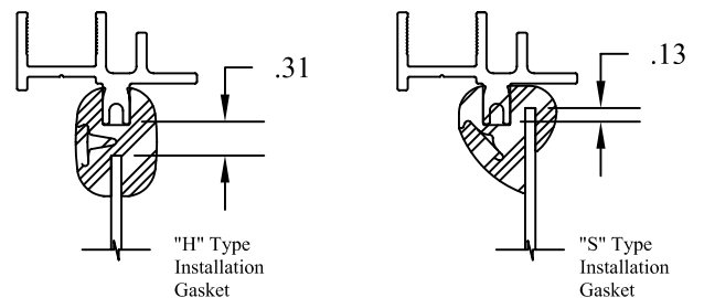
FIG. A WINDOW OPENING CLEARANCES
