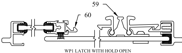
WP1 LATCH WITH HOLD OPEN
