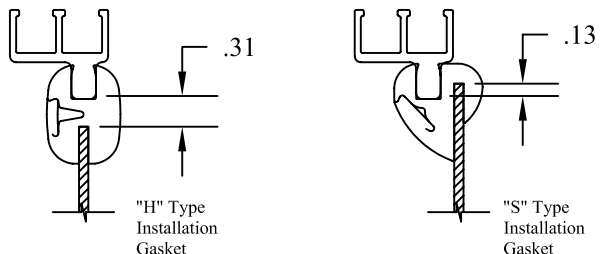
FIG. A WINDOW OPENING CLEARANCES
