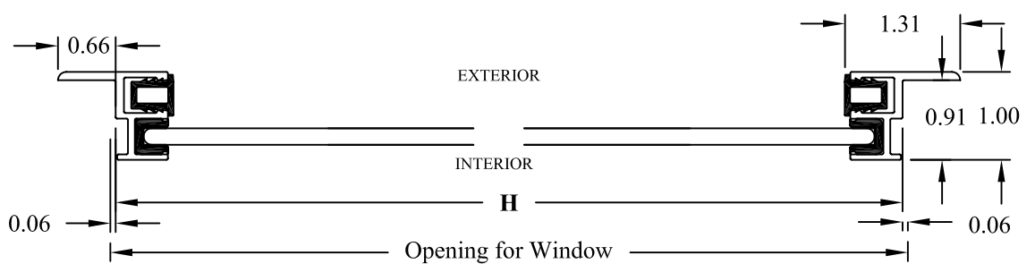
SECTION B-B
